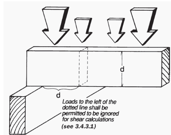
Figure 1. —Shear at supports. (Reprinted with permission from the American Forest & Paper Association, Inc.)
