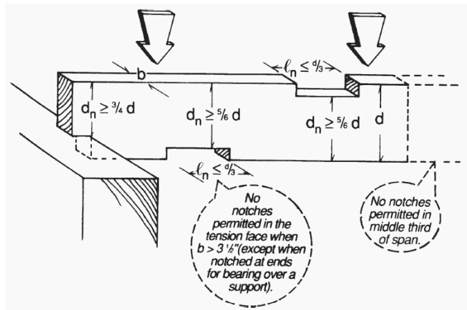
Figure 3.—Notch limitations for sawn lumber beams. (Reprinted with permission from the American Forest & Paper Association, Inc.)
