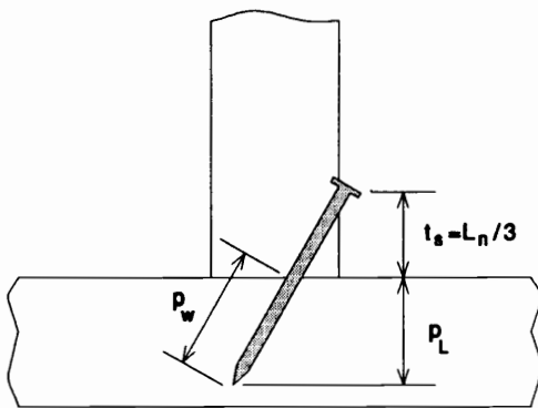
Figure C12.3-1 Effective penetration and side member thickness for toe nails subject to lateral loads.
